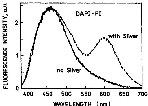
Fig. 3. Emission spectra of DNA labeled with both DAPI and PI between quartz plates (the control sample) and between silver island films. The emission spectra are normalized to the DAPI donor emission.
