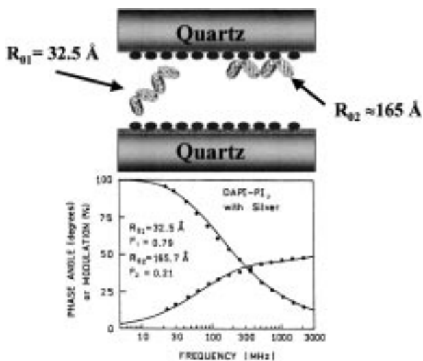
Fig. 4. Energy transfer analysis of the frequency-domain data in terms of two populations of DAPI-PI labelled DNA with different R_0 values. (Top)—Graphical representation of two DAPI-PI labelled DNA populations.
