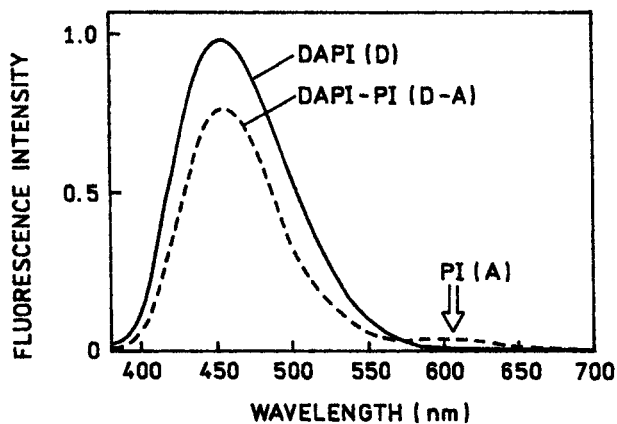
Fig. 2. Emission spectra of DNA labeled with DAPI and with DAPI and PI. The PI acceptor makes a very small contribution to the emission seen at 610 nm. D: Donor; A: acceptor molecule.
